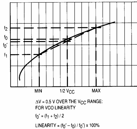
Figure 13B. Definition of VCO Frequency Linearity
