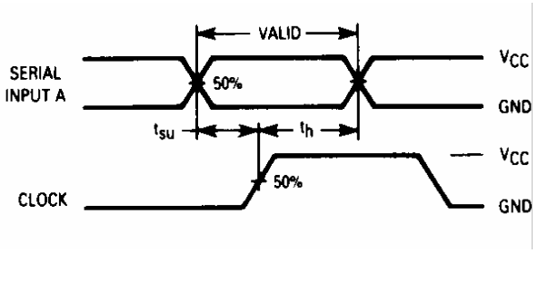
Figure 4. Switching Waveforms
