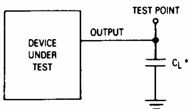
Figure 5. Test Circuit
