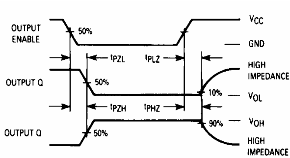
Figure 3. Switching Waveforms
