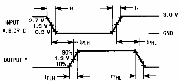
Figure 1. Switching Waveforms
