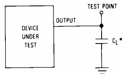
Figure 2. Test Circuit
