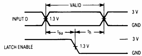
Figure 4. Switching Waveforms
