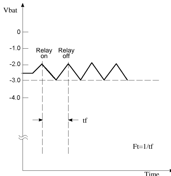
Fig. 8. One Defective Lamp Oscillator Timing Diagram
